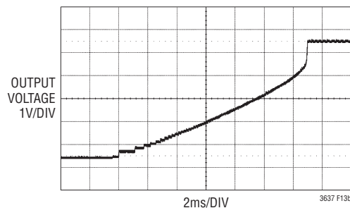
Soft-Start Waveform
