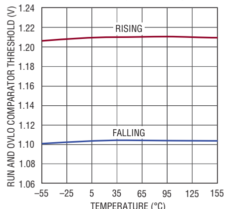
RUN and OVLO Comparator Threshold Voltages vs Temperature
