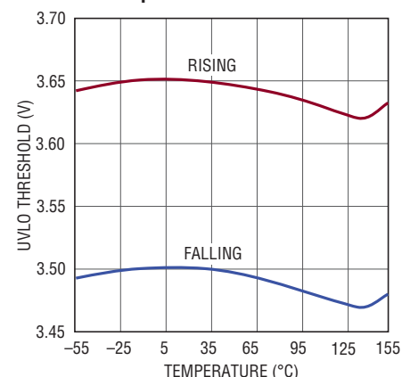
UVLO Threshold Voltages vs Temperature
