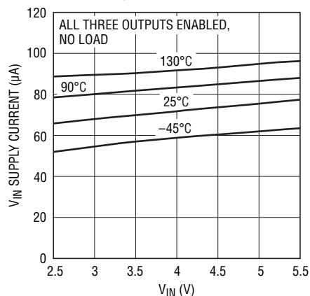
V_{IN} Supply Current vs V_{IN}
