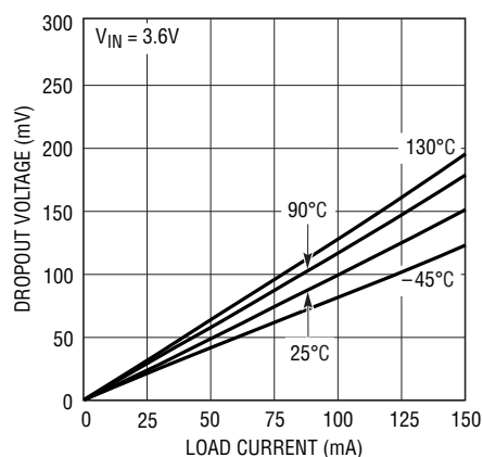
LDO Dropout vs Load Current at V_{IN} = 3.6\text{V}
