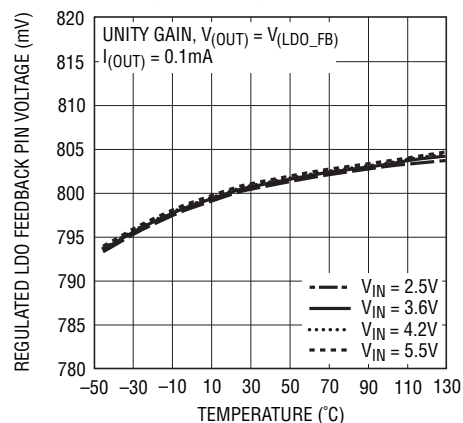
Regulated LDO Feedback Pin Voltage vs Temperature
