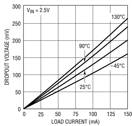
LDO Dropout vs Load Current at V_{IN} = 2.5\text{V}
