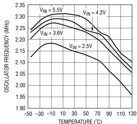
Buck Oscillator Frequency vs Temperature
