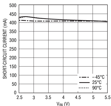
LDO Short-Circuit Current vs V_{IN}
