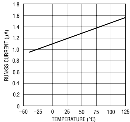
RUN/SS Current vs Temperature
