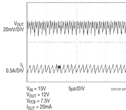
Constant Frequency (Burst Inhibit) Operation (Figure 12)
