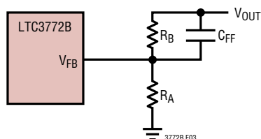
Figure 3. Setting Output Voltage
