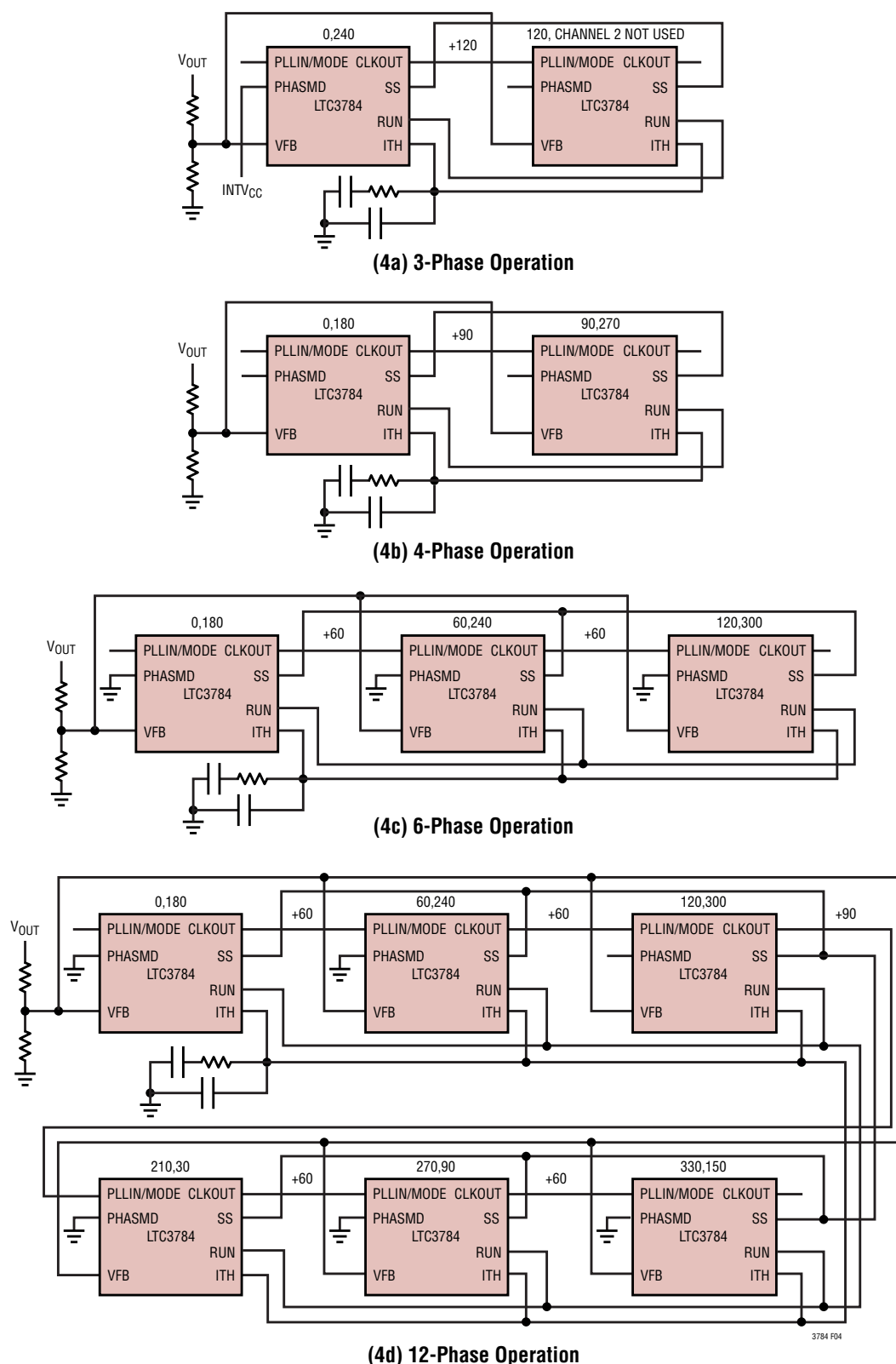
Figure 4. PolyPhase Operation
