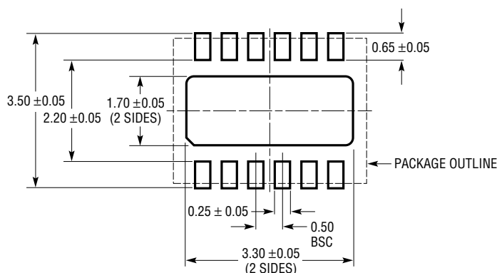
RECOMMENDED SOLID PAD PITCH AND DIMENSIONS
