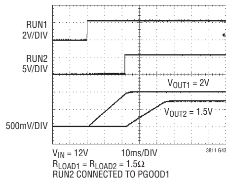
Sequenced Start-Up
