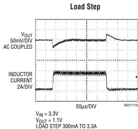
Figure 12. Externally Synchronized 700kHz, 3.3V IN , 1.1V/8A Step-Down Converter
