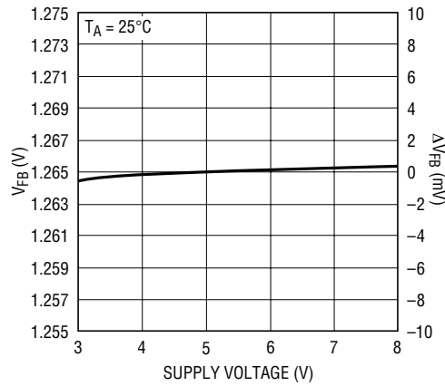
Line Regulation
