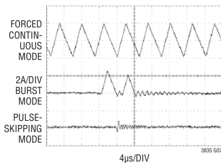
FIGURE 11 CIRCUIT V_{OUT} = 3.3\text{V} I_{LOAD} = 300\mu\text{A}
