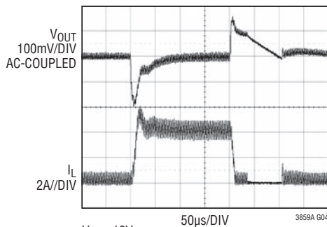
Load Step (Buck) Burst Mode Operation
