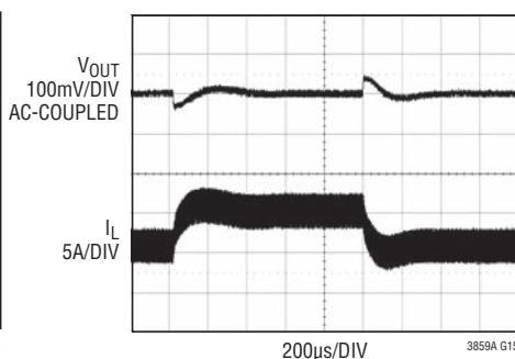
Load Step (Boost) Forced Continuous Mode
