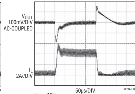
Load Step (Buck) Pulse-Skipping Mode
