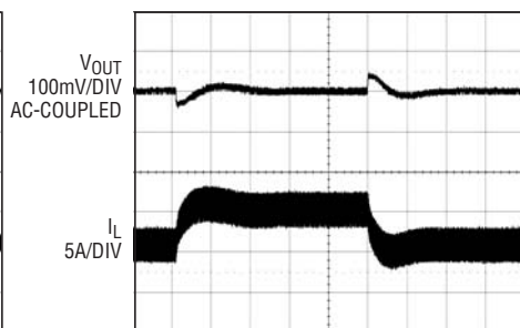
Load Step (Boost) Forced Continuous Mode
