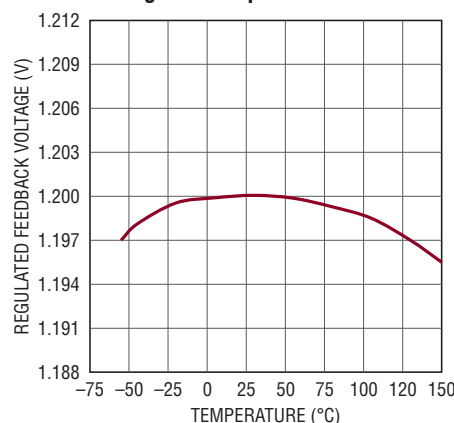
Boost Regulated Feedback Voltage vs Temperature
