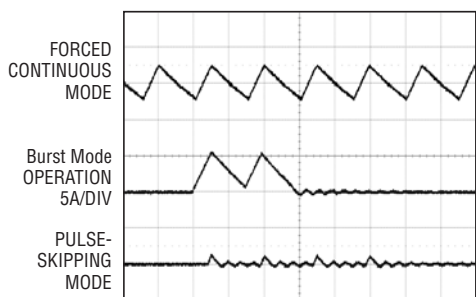
Inductor Current at Light Load (Boost)
