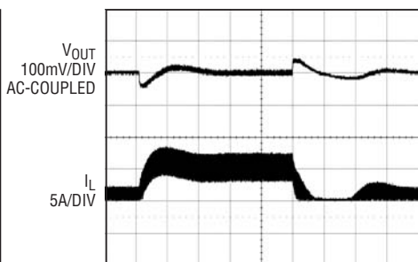
Load Step (Boost) Pulse-Skipping Mode
