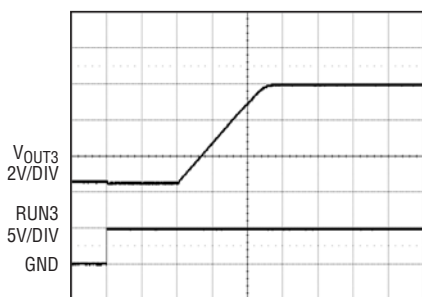
Soft Start-Up (Boost)
