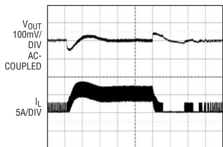
Load Step (Boost) Burst Mode Operation
