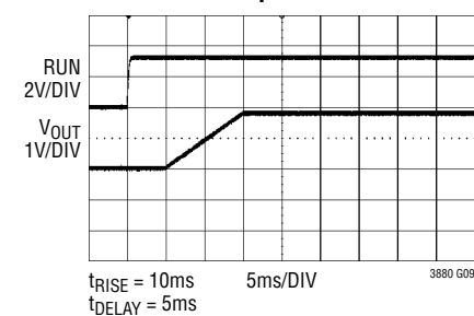
Soft-Start Ramp
