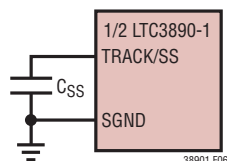
Figure 6. Using the TRACK/SS Pin to Program Soft-Start
