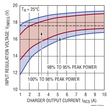
Solar Panel Input Regulation, Achieves Max Power Point to Greater than 98%
