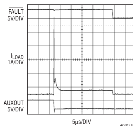
Figure 7. Short-Circuit Fault on 3.3V AUX Output
