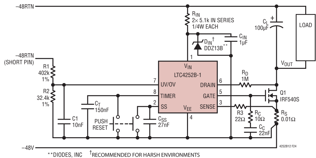
Figure 24. -48V/5A Application
