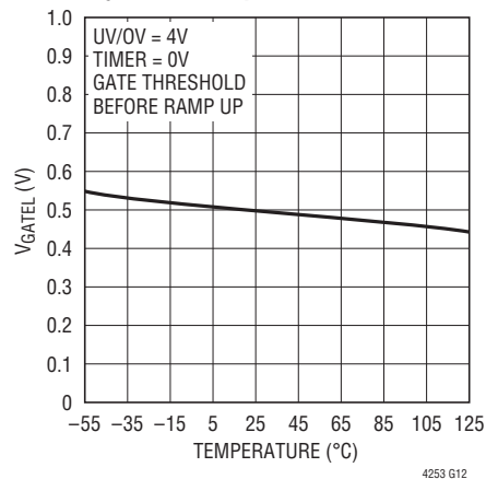
V_{GATEL} vs Temperature
