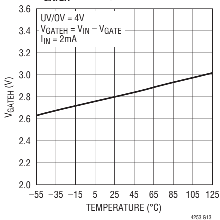
V_{GATEH} vs Temperature
