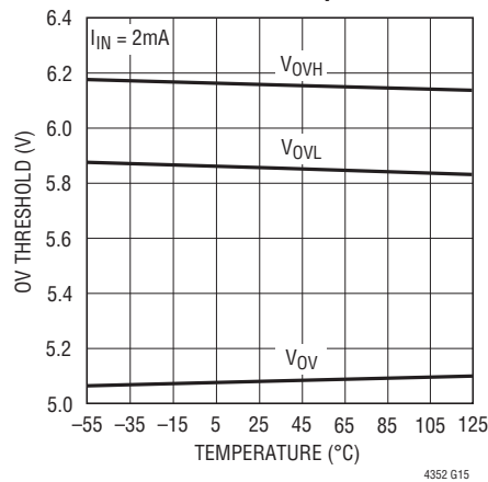
OV Threshold vs Temperature
