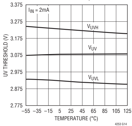
UV Threshold vs Temperature
