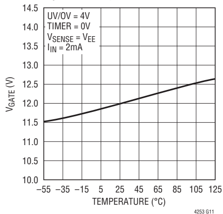
V_{GATE} vs Temperature
