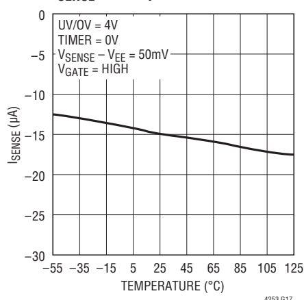
I_{SENSE} vs Temperature
