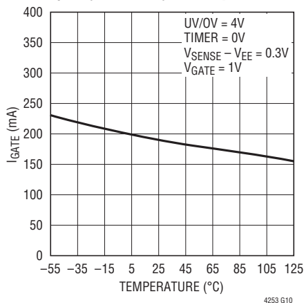
I_{GATE} (FCL, Sink) vs Temperature
