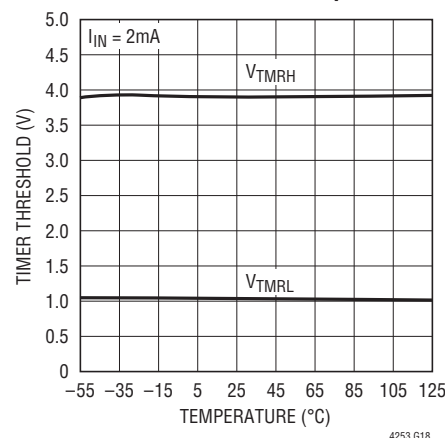
TIMER Threshold vs Temperature
