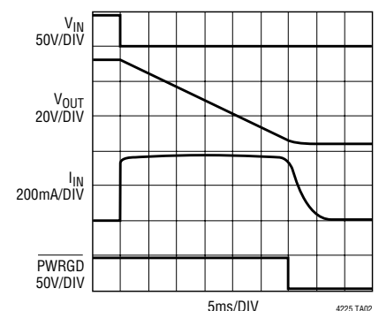
LTC4257 Charging 300μF Load Capacitor
