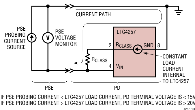
Figure 4. IEEE 802.af Measured-Voltage Method of Classification Probing
