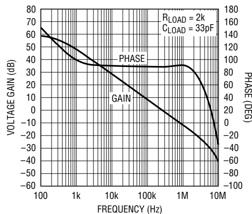
Figure 3. Measured Open Loop Gain and Phase, PCTL > 160\text{mV}
