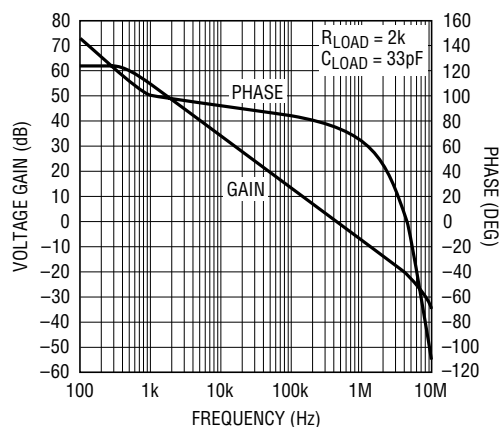
Figure 2. Measured Open Loop Gain and Phase, PCTL < 80\text{mV}
