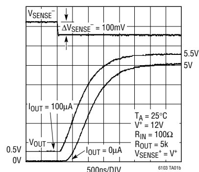
Step Response
