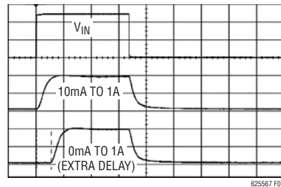
Figure 7. Time Domain Response Showing 2μs Rise Time. Top Waveform Is V_{IN} . Middle Waveform Is the 10mA to 1A Step Measured at R3, then the 0mA to 1A Step Showing Extra 2.7μs Delay When Recovering From 0mA
