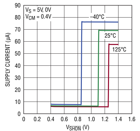
Supply Current vs \overline{\text{SHDN}} Pin Voltage
