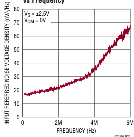
Wide Band Noise Voltage Density vs Frequency
