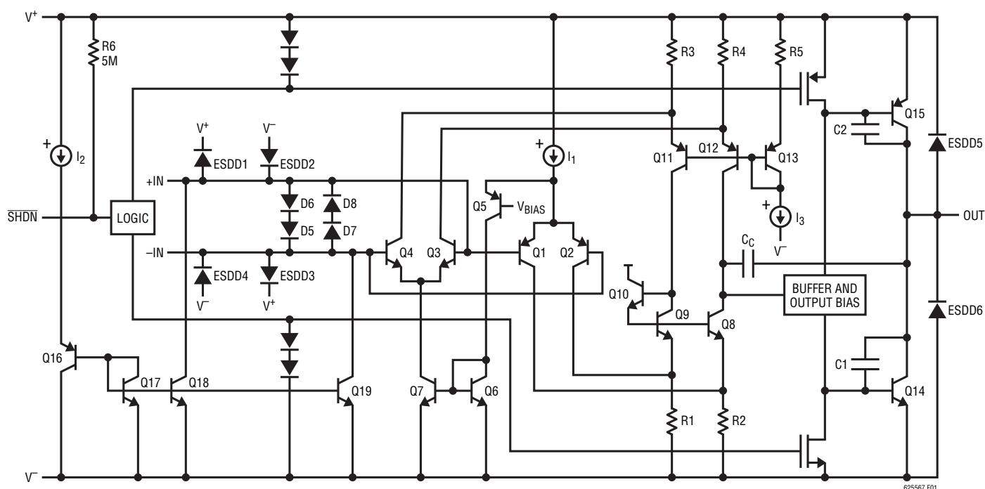
Figure 1. LTC6255/LTC6256/LTC6257 Simplified Schematic
