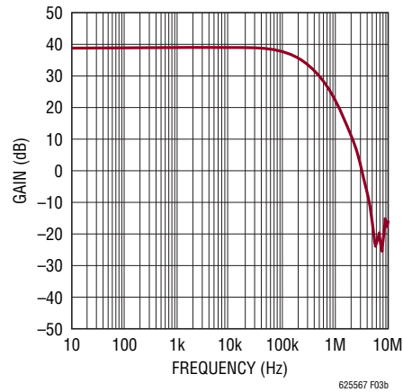
Figure 3. Gain of 100 Amplifier (3dB Bandwidth of 200kHz on 130 \mu A Supply Current)
