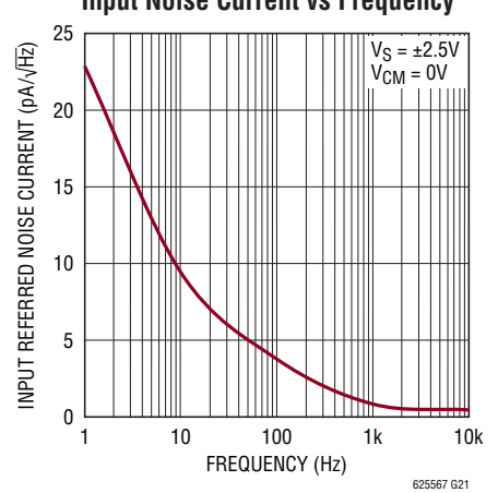
Input Noise Current vs Frequency
