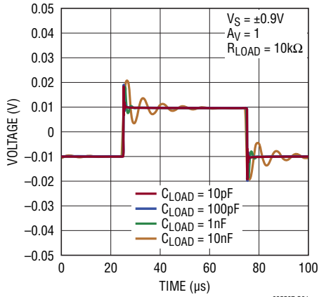
Small-Signal Response
