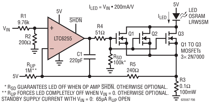
2μs Rise Time Analog 1A Pulsed LED Current Driver
