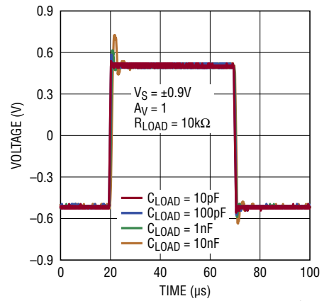
Large-Signal Response
