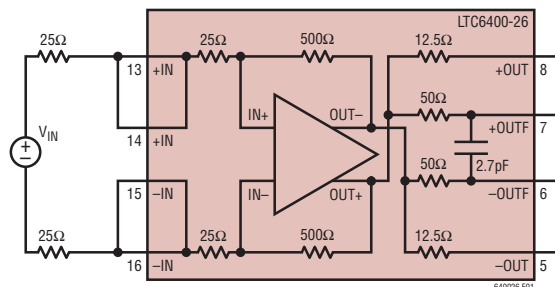
Figure 1. Input Termination for Differential 50Ω Input Impedance
