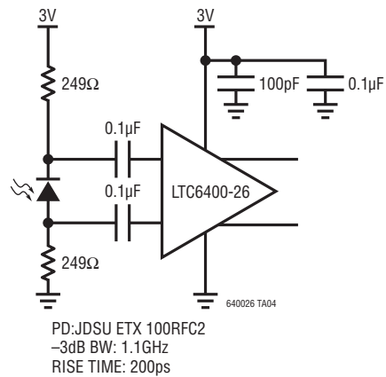
Optical Photodiode Receiver
