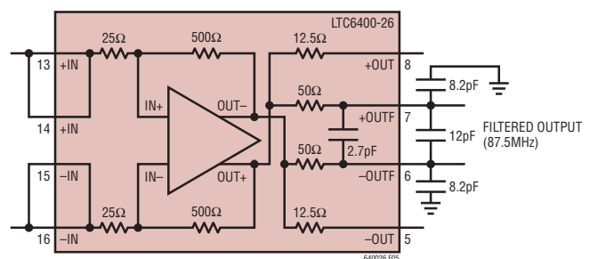
Figure 5. LTC6400-26 Internal Filter Topology Modified for Low Filter Bandwidth (Three External Capacitors)
