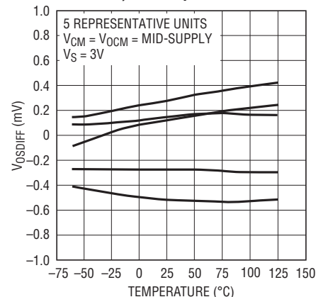
Differential Voltage Offset (Input Referred) vs Temperature
