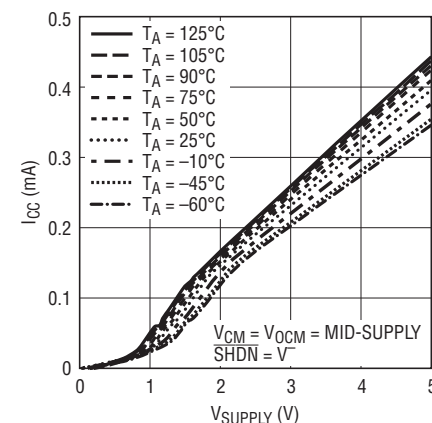
SHDN Supply Current vs Supply Voltage and Temperature
