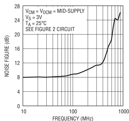
LTC6404-4 Noise Figure vs Frequency
