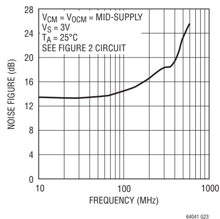
LTC6404-1 Noise Figure vs Frequency
