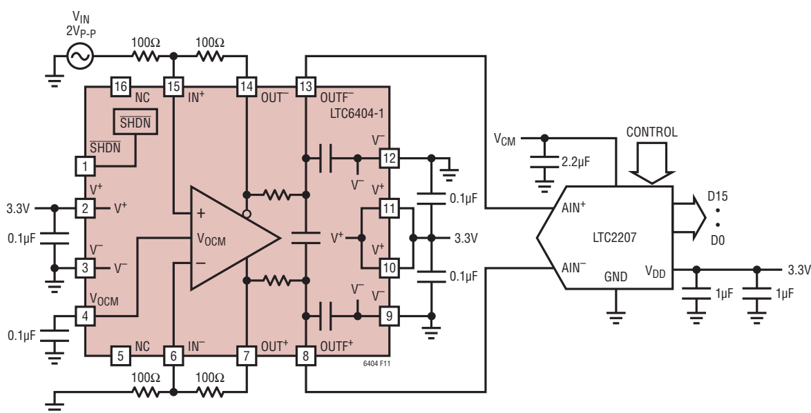
Figure 11. Interfacing the LTC6404-1 to a High Speed 105Msps ADC
