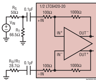
Figure 3. Input Termination for Single-Ended 50\Omega Input Impedance
