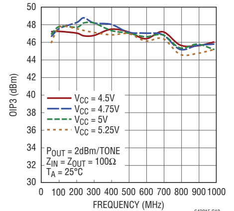
OIP3 vs Frequency Over V_{CC} Voltage
