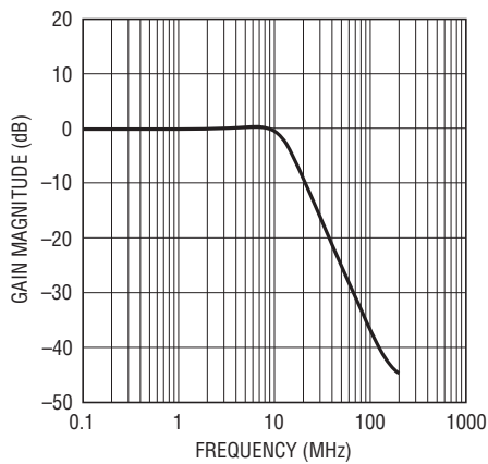
Gain Response
