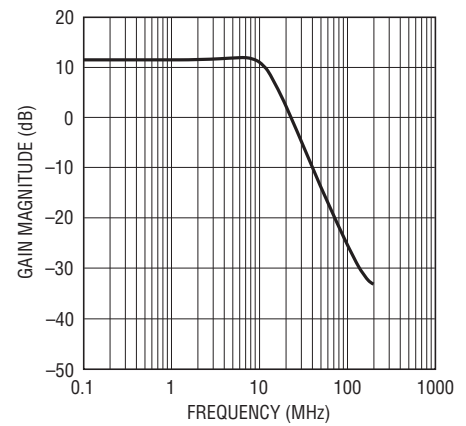
Gain Response
