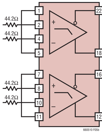
660510 F05b \pm 0.7\text{dB} 11.2MHz PASSBAND GAIN = 2.774\text{V/V} (8.9dB) Z_{\text{IN}} = 288\Omega
