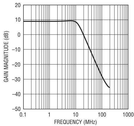
Gain Response
