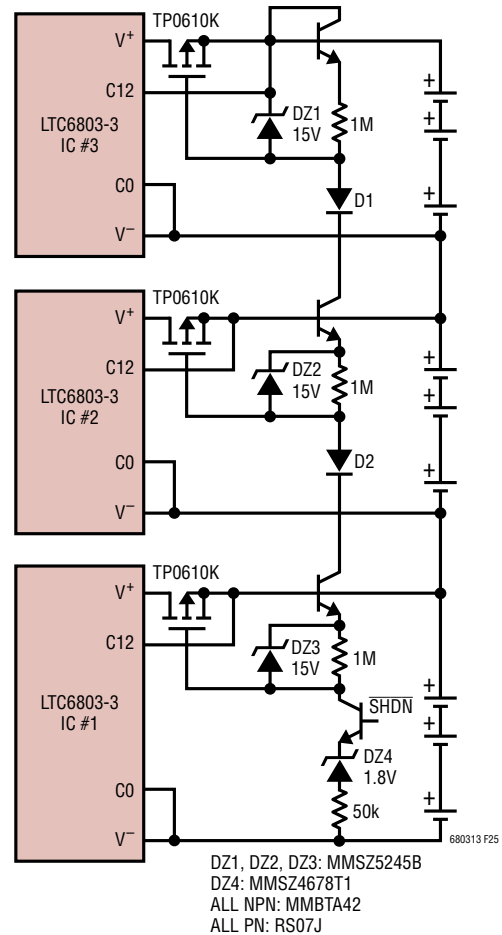
Figure 25. Hardware Shutdown Circuit Reduces Total Supply Current of LTC6803 to Less Than 1nA
