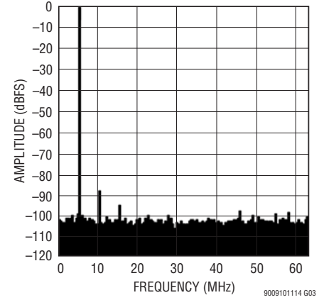
LTM9011-14: 8k Point FFT, f_{IN} = 5\text{MHz} , -1\text{dBFS} , 125Mps
