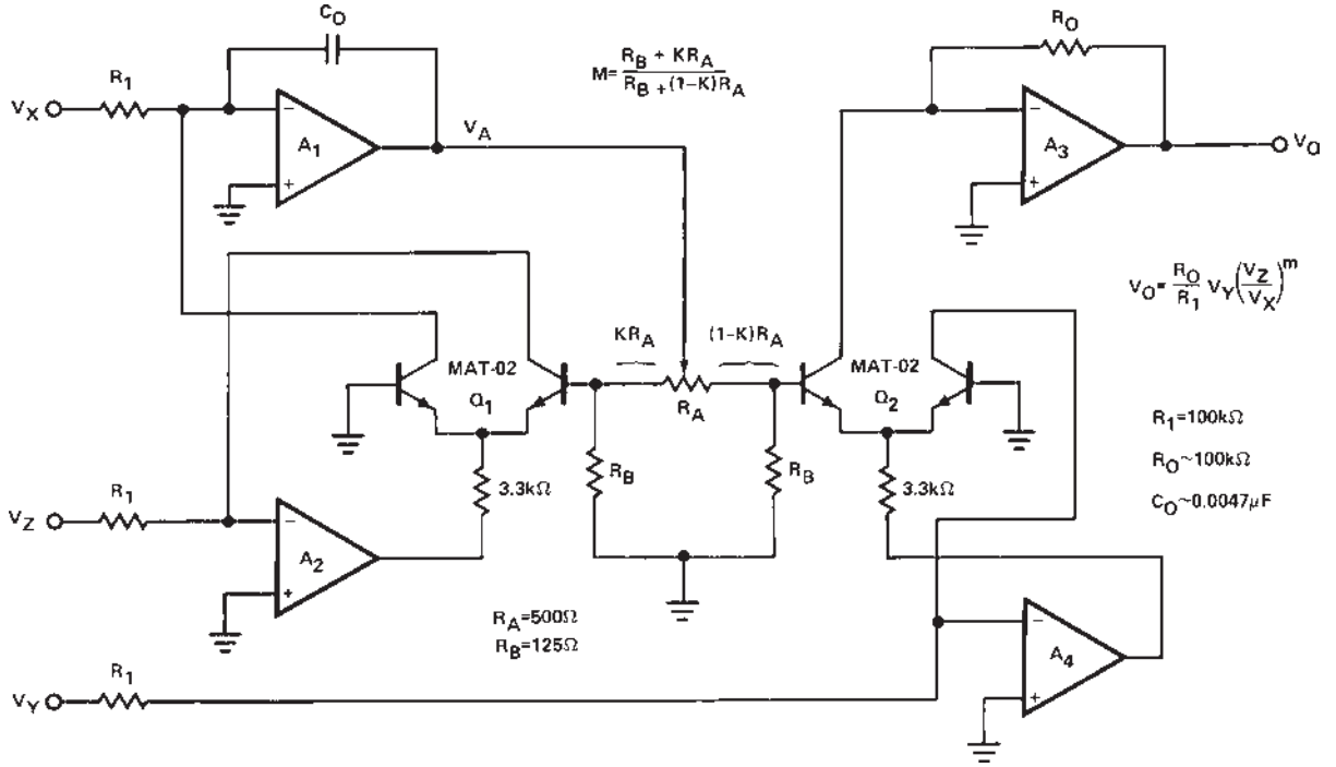
Figure 6. Multifunction Converter
