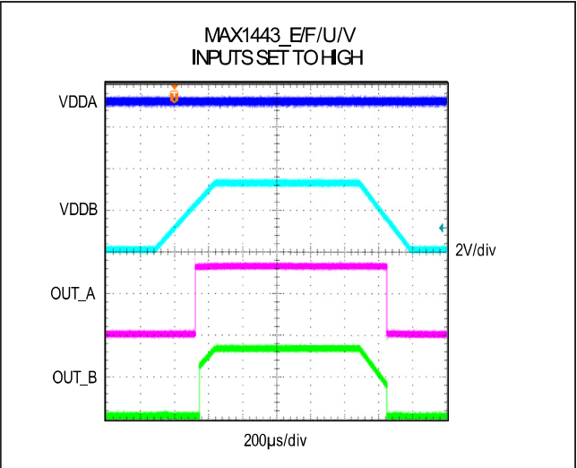
Figure 5. Undervoltage Lockout Behavior (MAX1443_E/F/U/V High)
