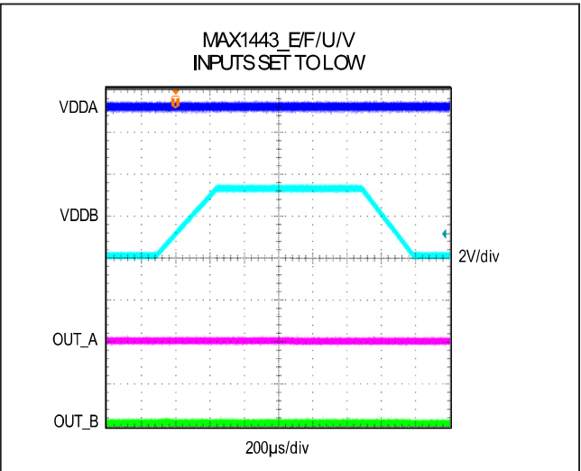
Figure 7. Undervoltage Lockout Behavior (MAX1443_E/F/U/V Low)
