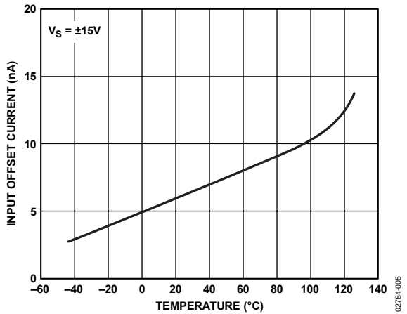
Figure 4. Input Offset Current vs. Temperature
