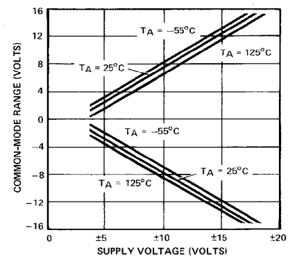
COMMON-MODE INPUT RANGE vs SUPPLY VOLTAGE
