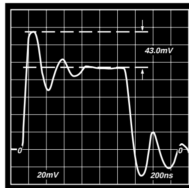
Figure 18. Small Signal Response; R_L = 2\text{ k}\Omega , C_L = 300\text{ pF} , V_S = \pm 2.5\text{ V} , A_V = +1 , V_{IN} = 100\text{ mV p-p}
