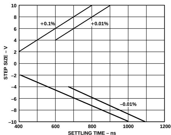
Figure 33. Settling Time vs. Step Size
