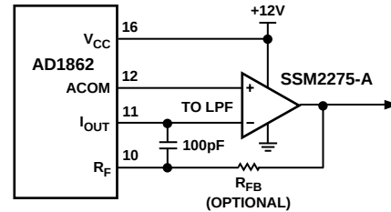
Figure 40. A High Performance I-V Converter for a 20-Bit DAC
