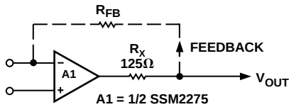
Figure 29. Output Short Circuit Protection Configuration
