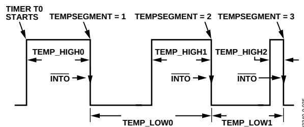
Figure 32. Reference Diagram for Software Variables in TMP05 Program Code Example 1
