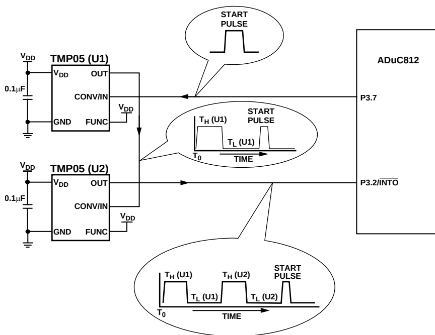
Figure 33. Typical Daisy-Chain Application Circuit
