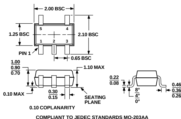
Figure 38. 5-Lead Thin Shrink Small Outline Transistor Package [SC-70] (KS-5)
