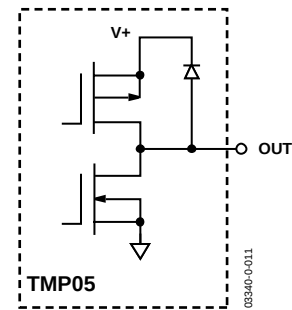
Figure 29. TMP05 Digital Output Structure
