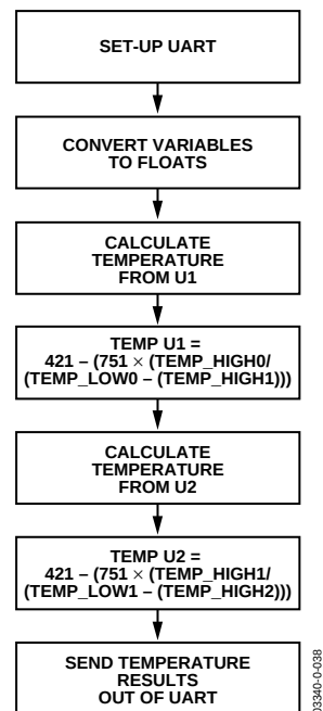
Figure 35. ADuC812 Temperature Calculation Routine Flowchart
