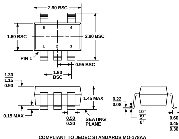
Figure 39. 5-Lead Small Outline Transistor Package [SOT-23] (RJ-5)
