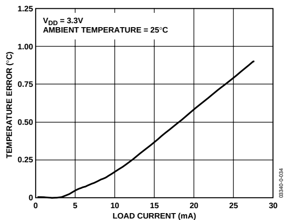
Figure 20. TMP05 Temperature Error vs. Load Current
