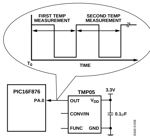
Figure 37. Typical Daisy-Chain Application Circuit
