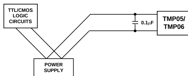
Figure 31. Use Separate Traces to Reduce Power Supply Noise
