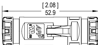
Mated View - Plug & Receptacle
