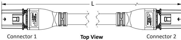
Connector 1 Top View Double Ended Plug Assembly
