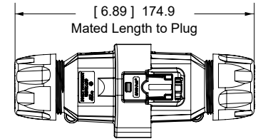
Mated View
