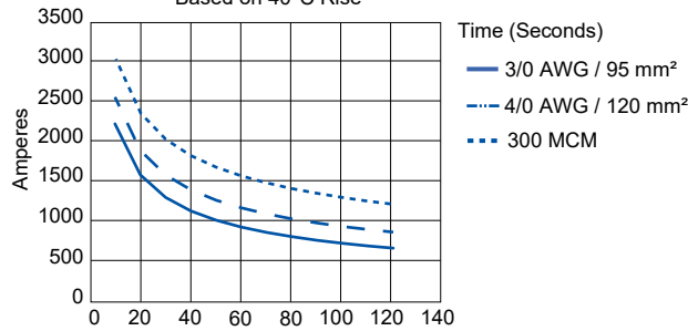
SBE® 320 / SBX® 350 InRush Current Curve Based on 40°C Rise
