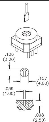
Arrow shaped slot
