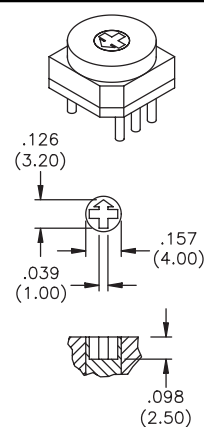
Cross shaped slot
