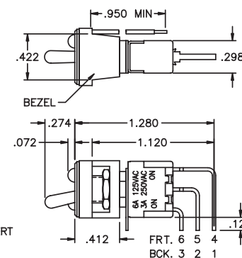
J94-ONE LED
