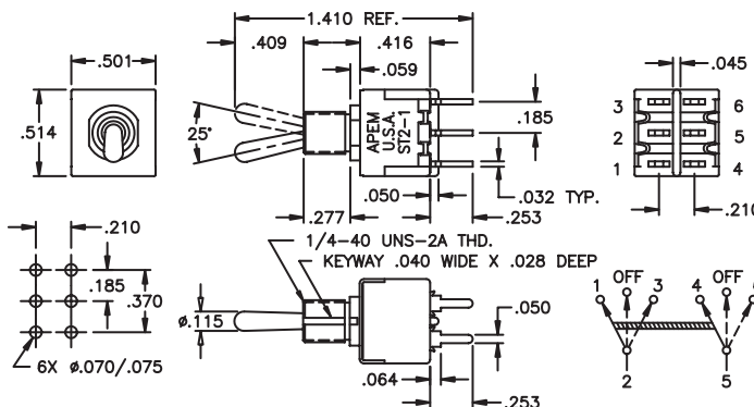
DOUBLE POLE
