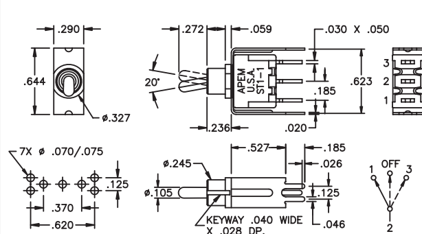
SINGLE POLE
