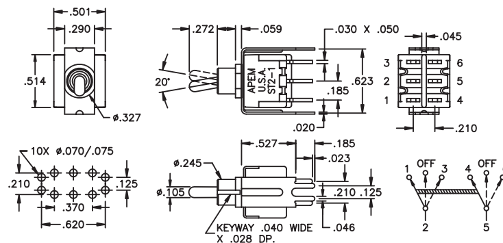
DOUBLE POLE
