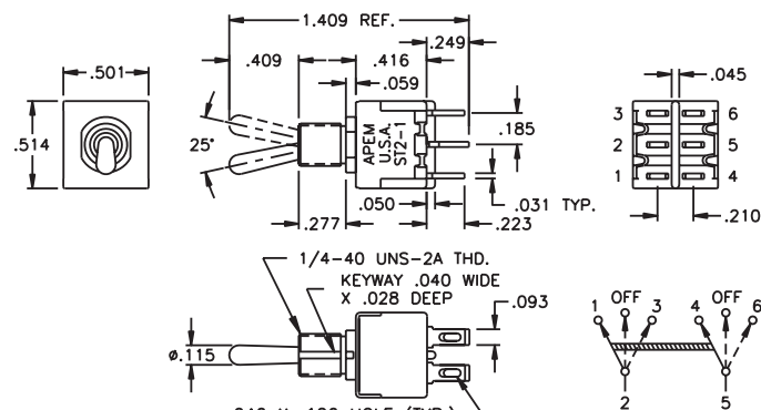
DOUBLE POLE
