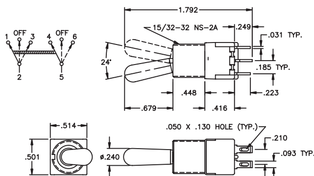
DOUBLE POLE
