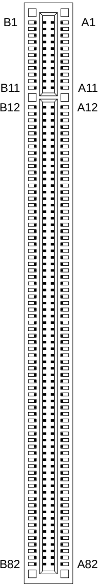
Figure 3-8: PCIe x16 slot connector pinout
