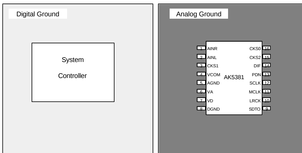
Figure 5. Ground Layout
