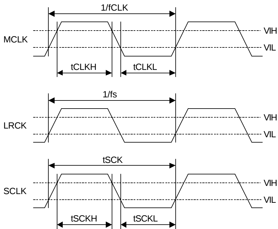
Clock Timing
