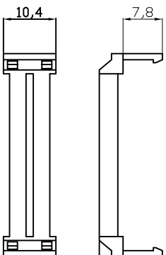
Strain Relief
