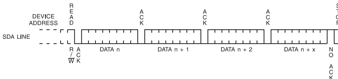
Figure 8-6. Sequential Read
