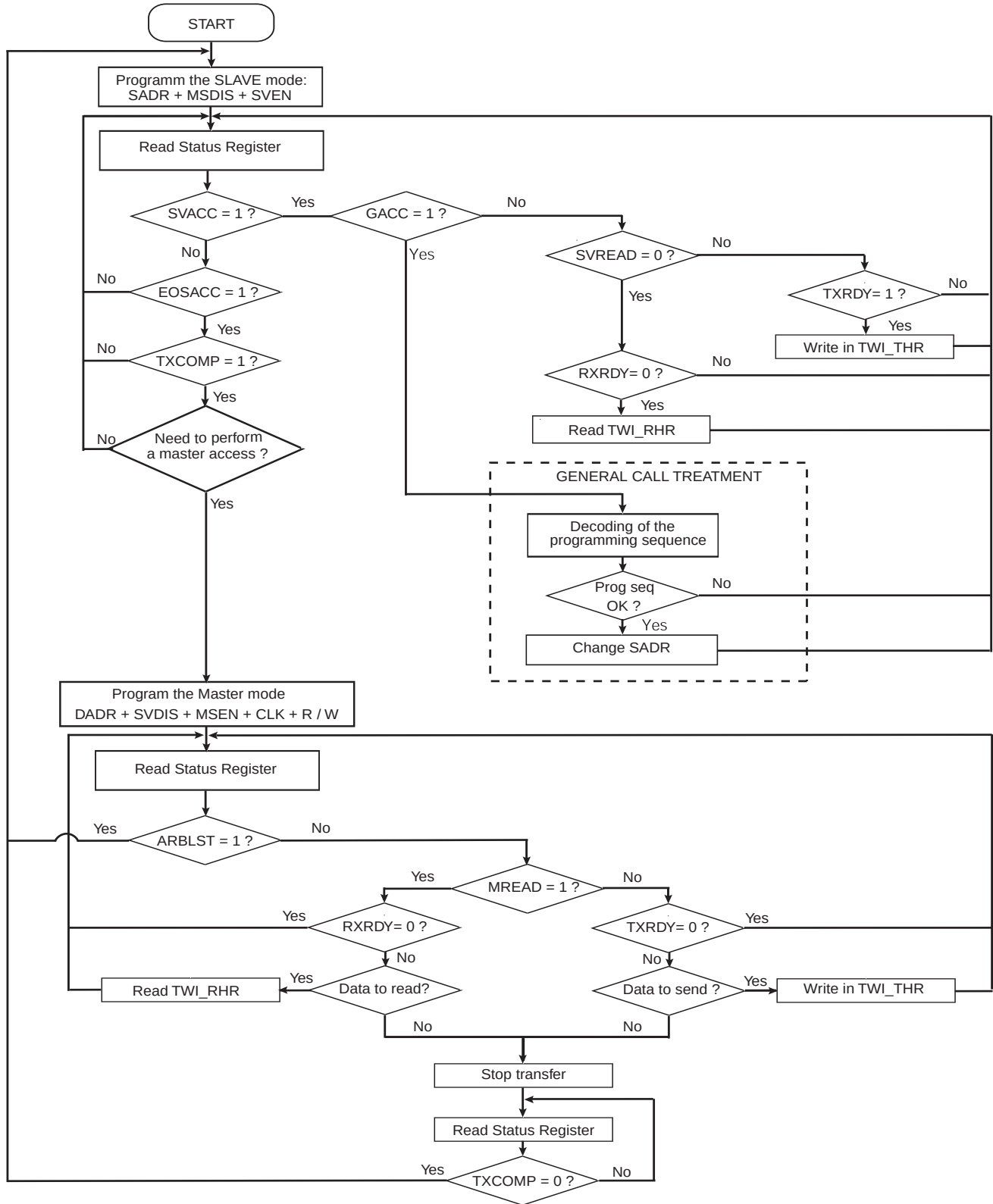
Figure 29-22. Multi-master Flowchart
