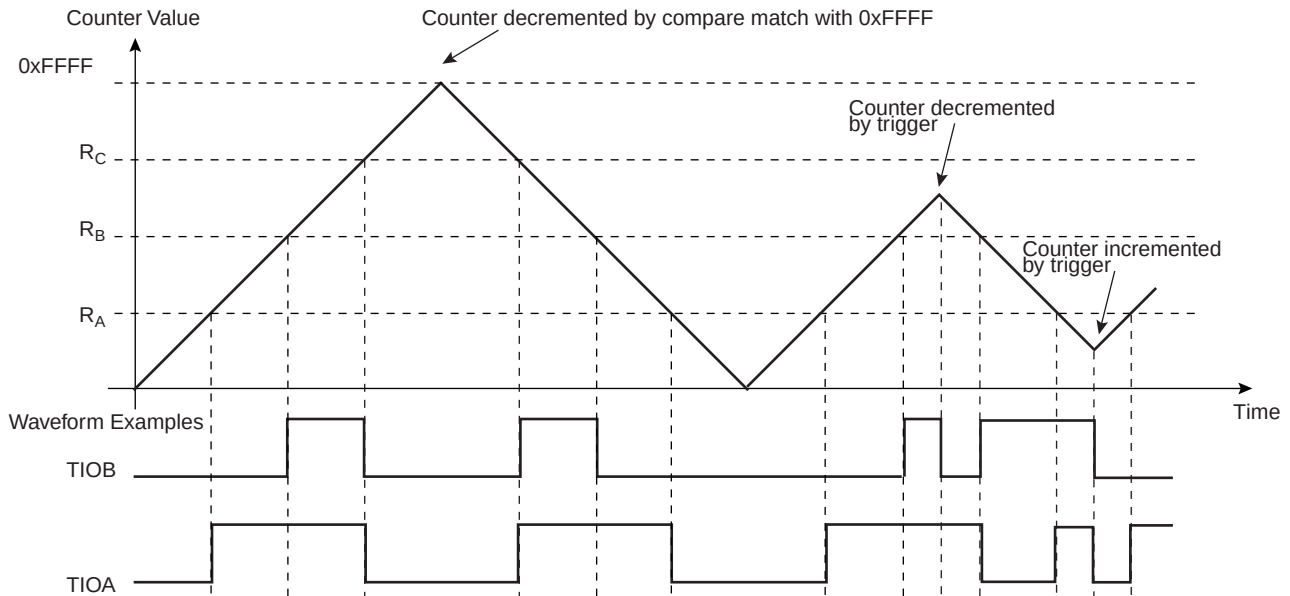
Figure 31-12. \overline{WAVSEL} = 01 With Trigger
