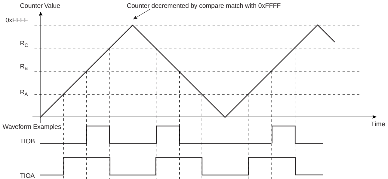
Figure 31-11. \overline{WAVSEL} = 01 Without Trigger
