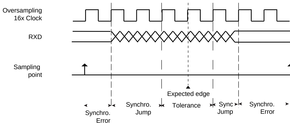
Figure 30-11. Bit Resynchronization
