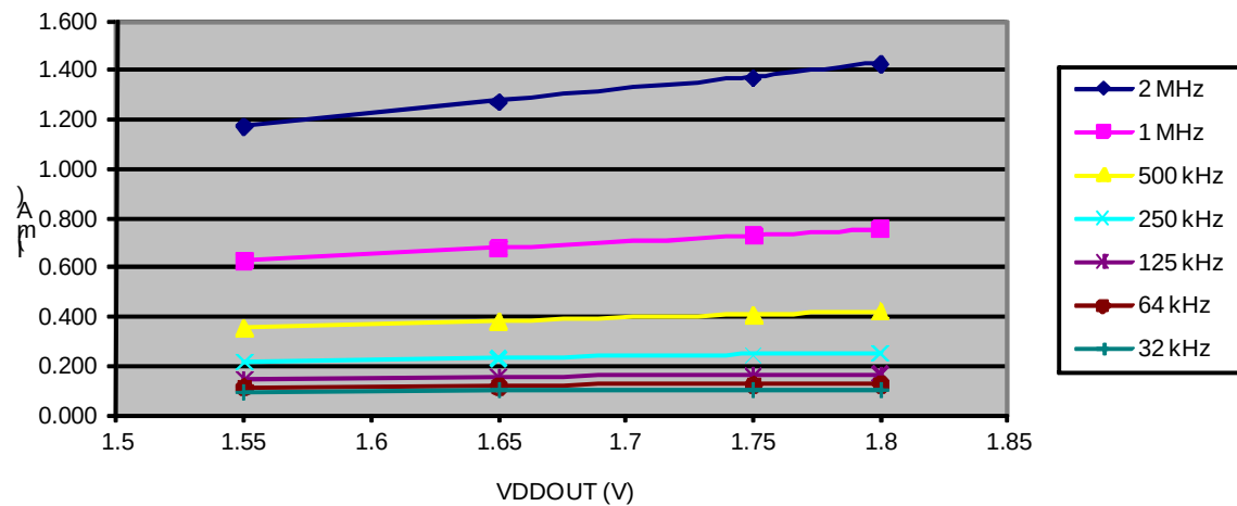
Figure 35-5. Low-range Frequencies, Active Mode Consumption @85°C (Peripheral Clocks On - PLL Off - RC On - VDD0I1 = 3V)
