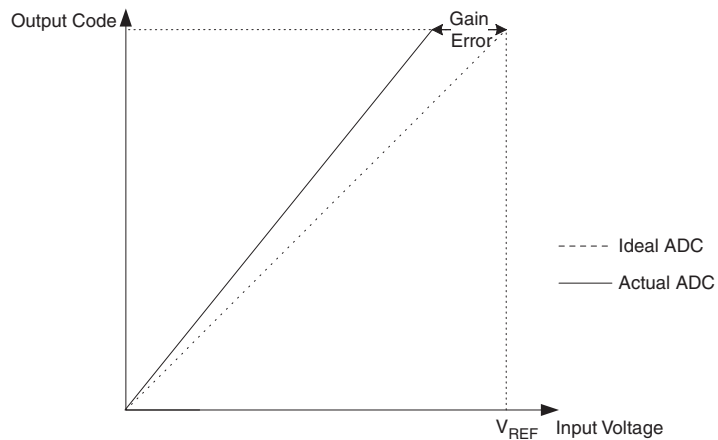
Figure 21-11. Gain Error
