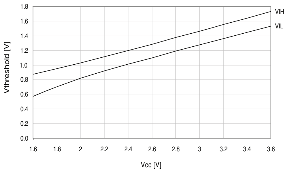
Figure 37-117. I/O pin input threshold voltage vs. V_{CC} .
