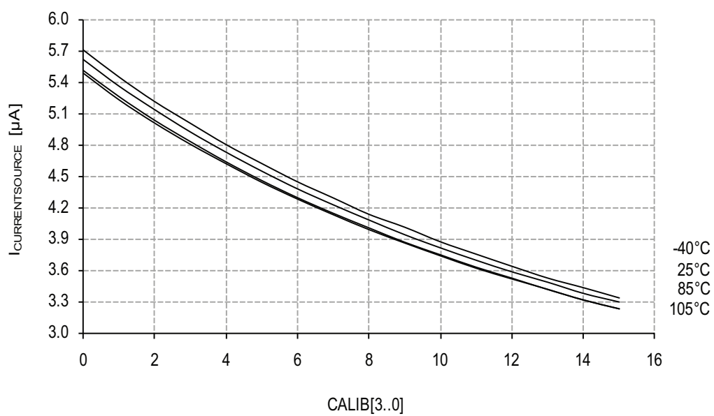
Figure 38-56. Analog comparator current source vs. calibration value.
