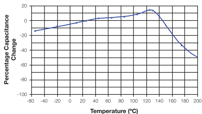
Typical Extended Temperature TCC Characterization of VHT, SMPS Capacitors Test conditions: 1 Vrms, 1 kHz, 0 VDC bias
